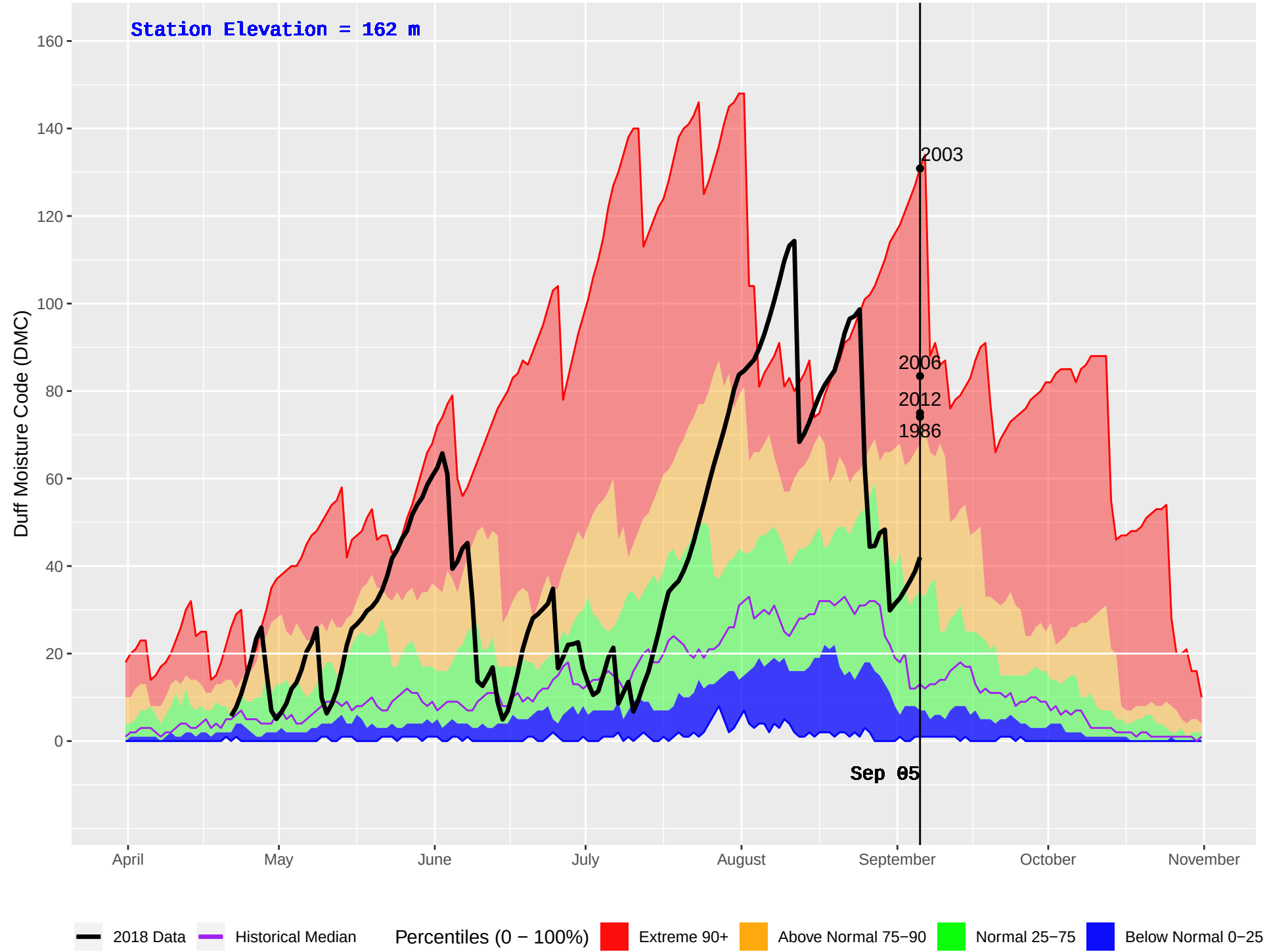
UBC RESEARCH (72) : Historical (1981–2016) and Current (2018) Daily Duff Moisture Code (DMC)
